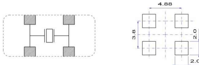
Example for soldering pattern
